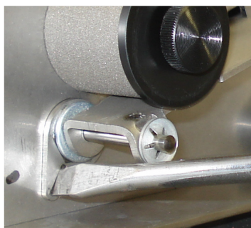
Fig 6 Screwdriver control
